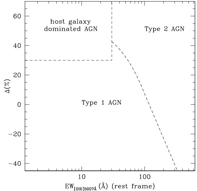
Fig. 8. Typical regions occupied by the XBS AGNs on the 4000\text{\AA} break/ [\text{OIII}]\lambda 5007\text{\AA} EW plot
