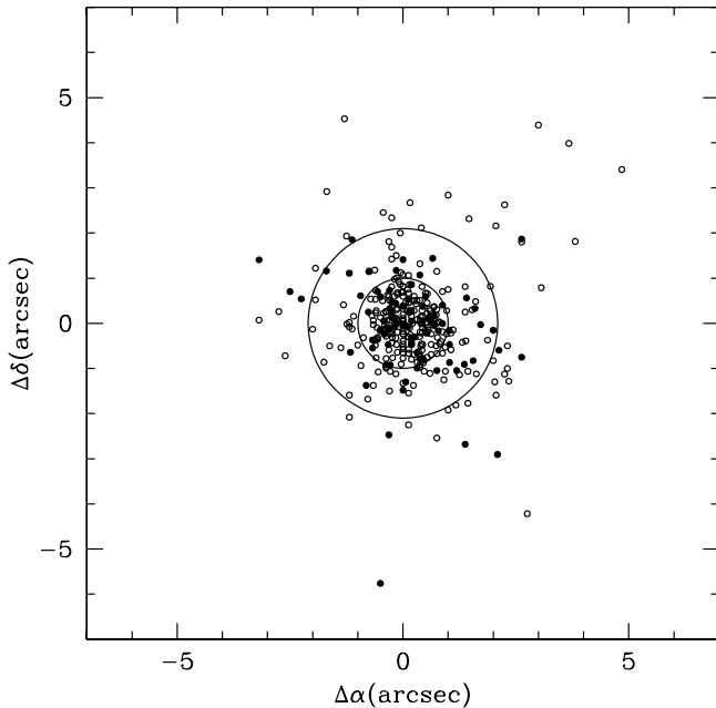
Fig. 3. X-ray/optical positional offsets of the XBS sources in common with the 2XMM catalogue (343 in total). In this case the X-ray positions are taken from the 2XMM catalogue that has been produced with recent versions of the Standard Analysis System. Symbols and regions as in Fig. 2
