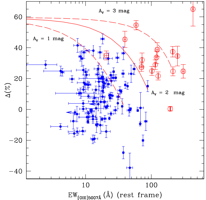
Fig. 6. 4000Å break ( \Delta ) versus the [OIII] \lambda 5007\text{\AA} equivalent widths for the BSS type 1 (filled points) and type 2 (open circles) AGNs, excluding the elusive ones. The three lines show the expected regions corresponding to different optical absorptions, from A_V=1 mag to A_V=3 mag, assuming a 10 Gyr early-type host galaxy
