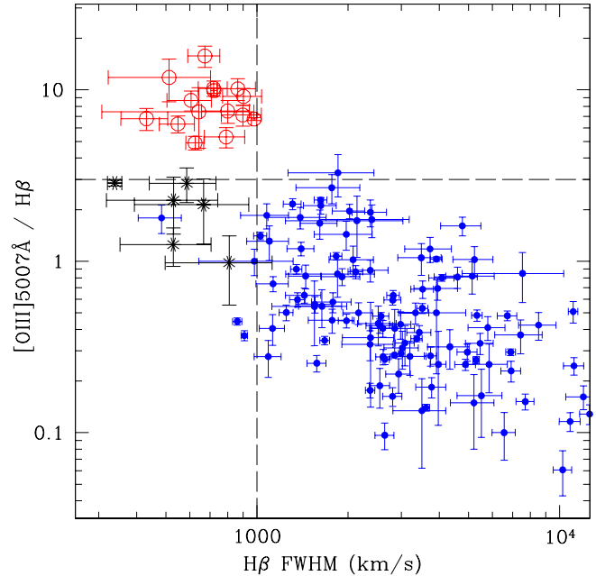
Fig. 5. [\text{OIII}]\lambda 5007\text{\AA} / \text{H}\beta flux ratio versus the \text{H}\beta emission line width for the sources in the XBS survey for which these lines have been detected ( z below \sim 0.65 ). Filled points are type 1 AGN, open circles are type 2 AGN, stars are objects spectroscopically classified as emission line galaxies (HII-region/starburst galaxies). The two dashed lines indicate the reference values used for the spectroscopic classification (see text and Fig. 4 for details)
