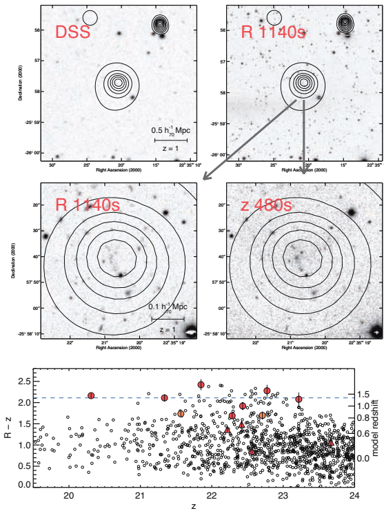
Figure 3 (left): Red-sequence detection technique applied to the cluster XMMU J2235.3-2557 at z = 1.39 . Top: X-ray flux contours overlaid on the DSS and FORS2 R (1140s) and z (480s) band images. The distant cluster is clearly extended in X-rays and lacks an optical counterpart in the DSS image. Bottom: Colour-magnitude diagram of the 7' \times 7' cluster centered field (AB magnitudes). Spectroscopically confirmed cluster galaxies at 1.38 < z < 1.40 are marked in red and 1.37 < z < 1.38 in orange. The location of the cluster red sequence calibrated by reasonable galaxy evolution models indicates a cluster redshift significantly beyond z = 1 .
