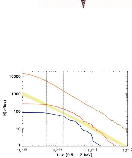
Figure 9 (below): Left: Expectations for the cluster detections as a function of redshift for a 14 \text{deg}^2 survey as calculated on the basis of the RDCS and 160 \text{deg}^2 surveys (Rosati et al. 2002, Mullis et al. 2004). The solid line gives the expectations for no evolution and the dashed line the more realistic predictions including the estimated evolutionary effects. Middle: Number counts as a function of detected flux in the best screened 12 \text{deg}^2 survey region: all detected X-ray sources (upper, orange line), all clearly extended sources (middle, red line), distant cluster candidates (lower, blue line). The yellow band indicates the logNlogS curve derived by Rosati et al. (2002) from the RDCS. Right: Distribution of the estimated photometric redshifts of the candidates from our pilot study.
