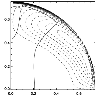
Fig. 11. The same as in Fig. 1 but with the effect of buoyancy, \text{Ra} = -2 \times 10^7 , \text{Rm} = 10^4 .
