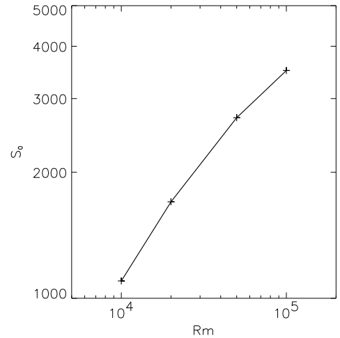
Fig. 9. Variation of S_0 with varying Rm as a log-log plot, for an approximate tachocline thickness of 0.028R_{\odot} .
