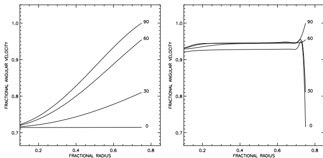
Fig. 3. Fractional \Omega vs. fractional radius for the initial configuration (left) and the equilibrium solution when B_{\text{pol}} is constant (right). Different lines represent \Omega at different co-latitudes.
