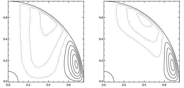
Fig. 10. Results for the simulations excluding (left) and including (right) buoyancy. The solid and the dotted lines are clockwise and anti-clockwise meridional circulation, respectively. \tilde{\text{Ra}} = -2 \times 10^7 , \text{Rm} = 10^4 .
