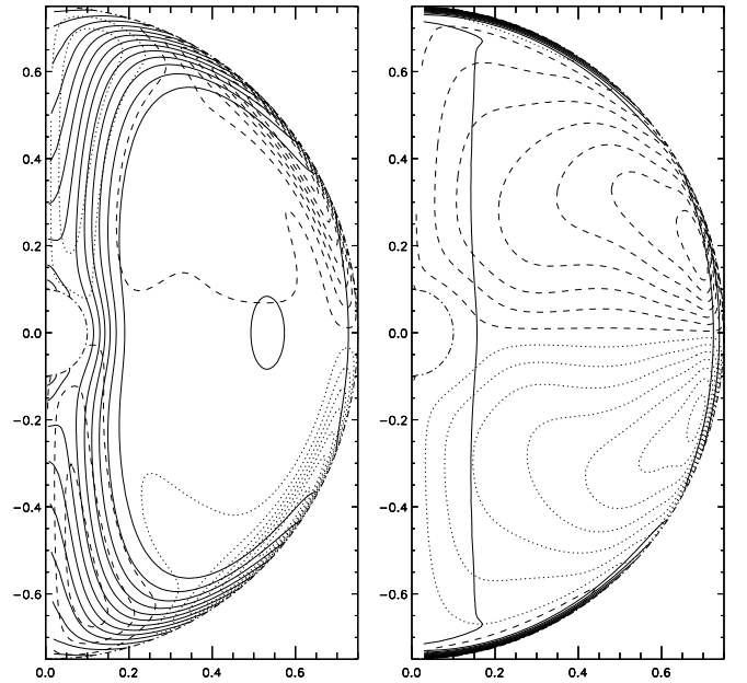
Fig. 1. Results for the simulations excluding (left) and including (right) the meridional circulation with the magnetic field being confined to the core. The solid lines are the iso-rotation curves, whereas the dashed and the dotted lines represent the contours of the positive and the negative toroidal field strength respectively. The dot-dashed lines indicate the boundaries of the simulation domain. The time-invariant poloidal magnetic field is not shown. S_0 = 1100 , Pm = 1 and Rm = 10^4 .
