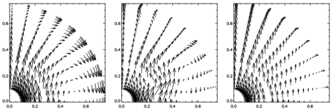
Fig. 5. Snapshots of B_{\text{pol}} in case of a decaying poloidal field at (from left to right) t = 0, 0.05\tau_{\text{diff}} , and 0.5\tau_{\text{diff}} . For every snapshot, length of arrows is proportional to the amplitude of B_{\text{pol}} at each point. The length of arrows is renormalized in each plot by corresponding maximum field amplitude. Only every fifth arrow in \theta and r is plotted in order to avoid congestion.
