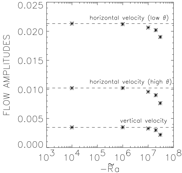
Fig. 12. Plot of the amplitudes of the components of the meridional flow at different co-latitudes \theta , normalized to the rotational velocity at the equator, with varying \tilde{Ra} . The dashed lines represent the corresponding values without buoyancy effect. Rm = 10^4 , Pm = 1 .
