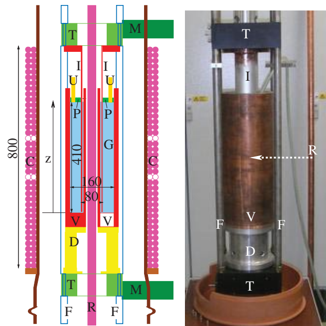
FIG. 1 (color). Sketch (left) and photograph (right) of the central module of the PROMISE facility. V —copper vessel, I —inner cylinder, G —GaInSn, U —two ultrasonic transducers, P —Plexiglas lid, T —high precision turntables, M —motors, F —frame, C —coil, R —central rod. The dimensions are in millimeters. When the experiment is running, the rod R in the right picture goes through the center of the cylinders.
