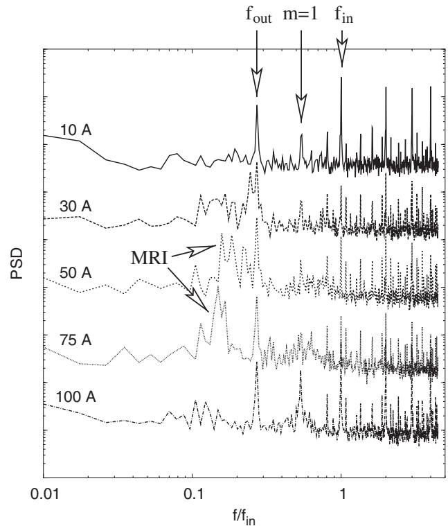
FIG. 3. Power spectra of the v_z fluctuations, averaged over 102 \text{ mm} < z < 190 \text{ mm} , for 5 different coil currents. The frequencies of the inner and outer cylinders are indicated. The MRI is visible at 50 and 75 A. In addition to that, an m = 1 mode is also present.
