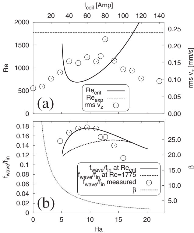
FIG. 4. (a) Computed critical Reynolds numbers and measured rms of the axial velocity, for varying I_{\text{coil}} (and hence Hartmann numbers), for fixed I_{\text{rod}} = 6000 A. (b) Frequency f_{\text{wave}} of the traveling MRI wave, normalized to the rotation rate f_{\text{in}} of the inner cylinder. The ratio of azimuthal field to axial field \beta is also shown.
