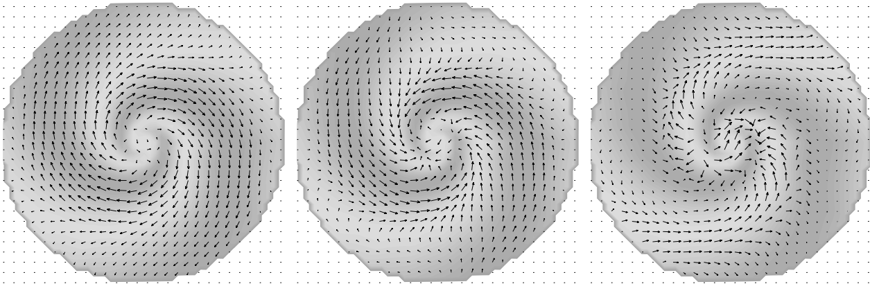
Fig. 2. Magnetic field geometry for LEFT: \tau_{\text{corr}} = 30 Myr (after 3.3 Gyr), MIDDLE: \tau_{\text{corr}} = 50 Myr (after 3.3 Gyr), RIGHT: \tau_{\text{corr}} = 100 Myr (after 2.0 Gyr). The optical spiral arms are shown in light grey.
