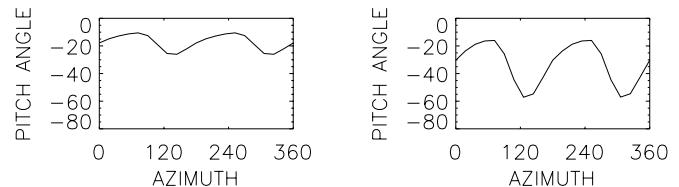
Fig. 3. Magnetic pitch angles in the mid-plane at r = r_{\text{max}}/2 for LEFT: \tau_{\text{corr}} = 30 Myr, RIGHT: \tau_{\text{corr}} = 50 Myr. (Both after 3.3 Gyr.)
