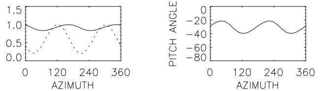
Fig. 7. A model with axisymmetric turbulence contribution ( Q_u = \text{const.} , cf. Eq. 15): LEFT: Normalized field strength (solid) compared with density profile (dotted), RIGHT: Magnetic pitch angles. \tau_{\text{corr}} = 50 Myr. Located in the mid-plane at r = r_{\text{max}}/2 , after 3.42 Gyr.
