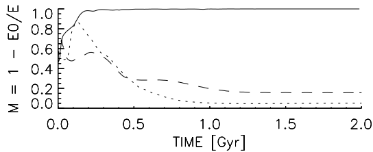
Fig. 5. Symmetry parameter M for \tau_{\text{corr}} = 100 Myr (solid) compared with the ASS type solutions for \tau_{\text{corr}} = 50 Myr (dashed) and \tau_{\text{corr}} = 30 Myr (dotted).
