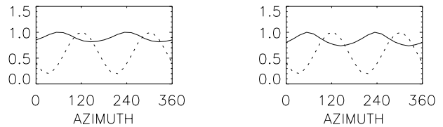
Fig. 4. Normalized field strength (solid) compared with density profile (dotted) for LEFT: \tau_{\text{corr}} = 30 Myr, RIGHT: \tau_{\text{corr}} = 50 Myr. (Position and time as in Fig. 3.)
