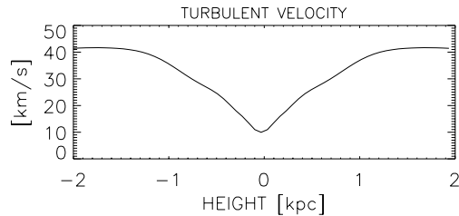
Fig. 1. The maximal turbulent velocity calculated from Eq. (16).
