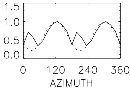
Fig. 6. Normalized field strength (solid) compared with density profile (dotted) in the mid-plane at r = r_{\text{max}}/2 for \tau_{\text{corr}} = 100 Myr (after 2 Gyr).
