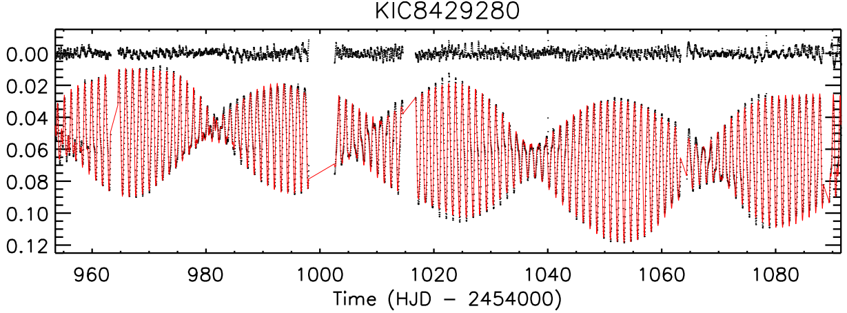
Fig. 7. Robust fit of the Kepler light curves. Q0 is from 953.53825 to 963.24461, Q1 from 964.51154 to 997.98296, and Q2 from 1002.76455 to 1091.46678. The solid line is the best fit of the first solution. The residuals, shown at the top, are \pm 2.36 mmag. The gaps are artificially bridged by straight connecting lines.
