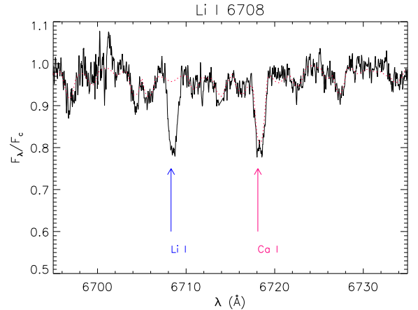
Fig. 4. Continuum-normalized spectrum (solid black line) in the lithium region of KIC 8429280 together with the template spectrum (dotted red line) of the non-active lithium-poor reference star, broadened at the v \sin i of the target and Doppler-shifted according to the RV difference.
