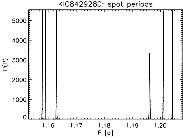
Fig. 8. Marginal distributions of spot periods. The two slowest revolving spots exhibit the same period. The periods group around two principal periods, which produces the obvious “beating” phenomenon quite understandable.
