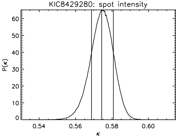
Fig. 10. Spot intensity with respect to the unspotted photosphere. Vertical lines mark the mean and the 68-per-cent confidence region.
