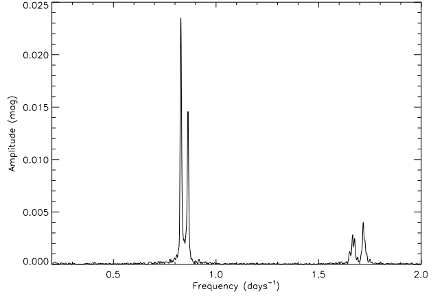
Fig. 6. Power spectrum of the Kepler Q0+Q1+Q2 time series of KIC 8429280.
