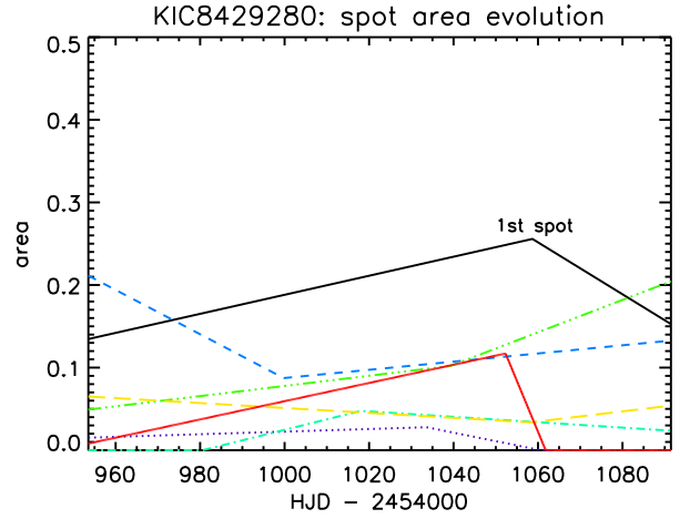
Fig. 12. Evolution of spot areas for the second solution. The different types of line have the same meaning as in Fig. 11.
