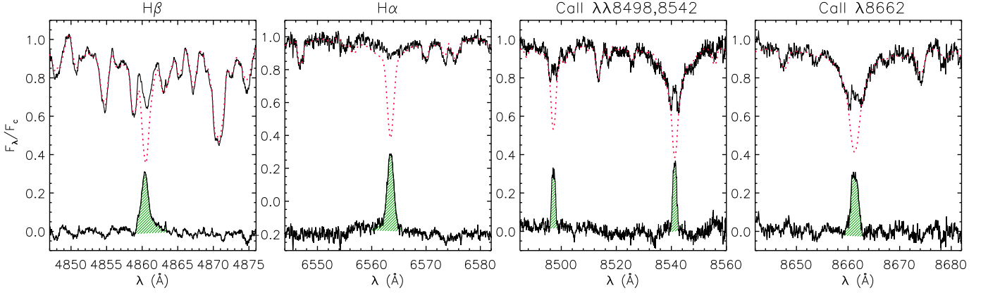
Fig. 3. Top of each panel: Observed, continuum-normalized SARG spectra of KIC 8429280 (solid line) in the H\beta , H\alpha , and Ca II IRT regions together with the non-active stellar template (dotted red line). Bottom of each panel: Difference between observed and template spectra. The residual H\alpha profile is plotted shifted downwards by 0.2 for the sake of clarity. The hatched areas represent the excess emissions that have been integrated to get the net equivalent widths.
