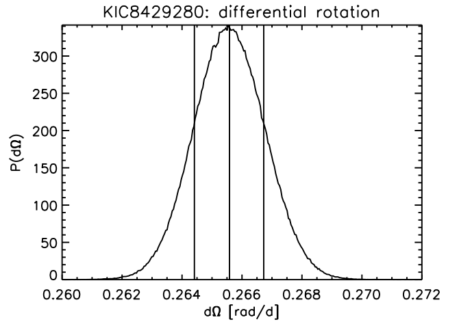
Fig. 13. The equator-to-pole differential rotation. Vertical lines mark the mean and the 68-per-cent confidence region.
