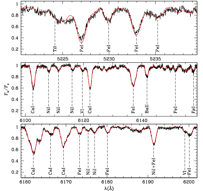
Fig. 1. Continuum-normalized observed spectrum (solid black line) in the region between 5220 and 5240 Å ( top panel ) and between 6100 and 6200 Å ( middle and bottom panels ) of KIC 8429280. The synthetic spectrum calculated with the parameters listed in Table 3 is superimposed (smooth red line).
