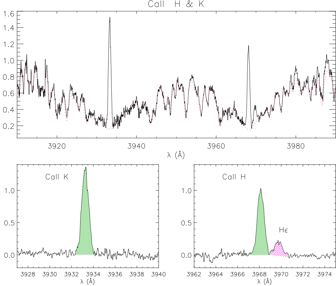
Fig. 2. Top panel: Continuum-normalized SARG spectrum of KIC 8429280 (solid line) in the Ca II H & K region together with the inactive stellar template (dotted red line) broadened at the v \sin i of the target and Doppler-shifted according to the RV difference. Bottom panels: The difference spectrum. H \epsilon emission, already apparent in the observed spectrum, is clearly emphasized in the residuals.
