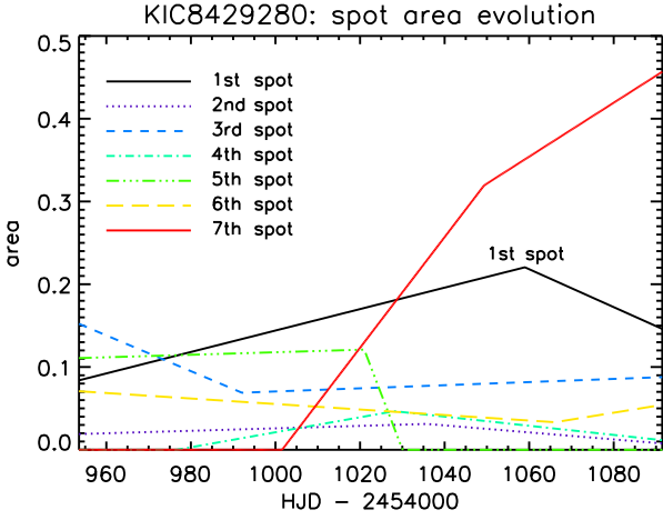
Fig. 11. Evolution of spot areas. Areas are expressed in units of the star’s cross-section. The largest spots are those at high latitudes.
