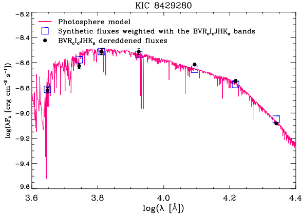
Fig. 5. Spectral energy distribution for KIC 8429280 (dots). The NextGen spectrum with T_{\text{eff}} = 5000 K and \log g = 4.0 is overplotted with a continuous line.
