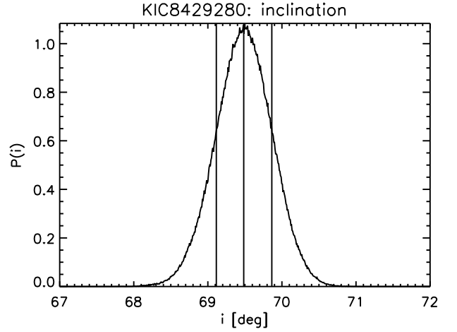
Fig. 9. The star’s inclination from Kepler photometry. Vertical lines mark the mean and the 68-per-cent confidence region. The inclination value confirms the relative large radius of the star.
