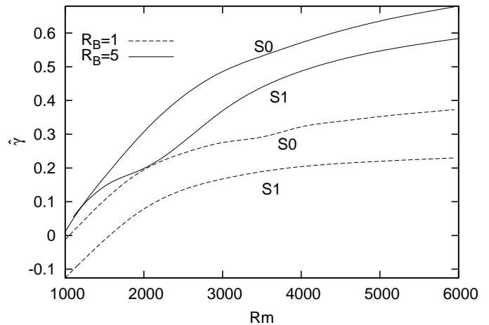
Fig. 2. \hat{\gamma} is a nondimensionalized growth rate ( \hat{\gamma} = \tau_{rot}\gamma , where \gamma is in physical units), of the S0 and S1 modes, for R_B = 1 and 5. The profiles for A0 and A1 are very similar, and are not shown here.
