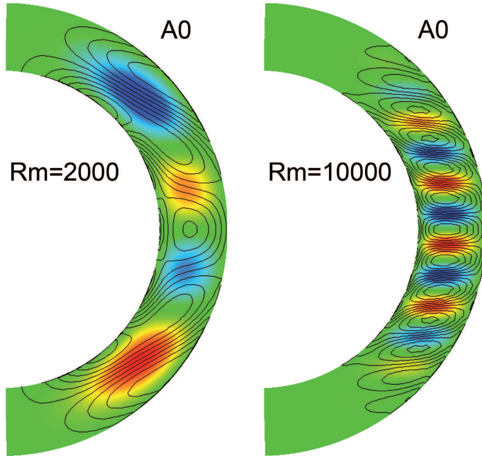
Fig. 3. The axisymmetric solution A0 for R_B = 1 , and Rm = 2000 on the left and Rm = 10000 on the right. The other modes have the same pattern of exhibiting finer structure in z for larger Rm .
