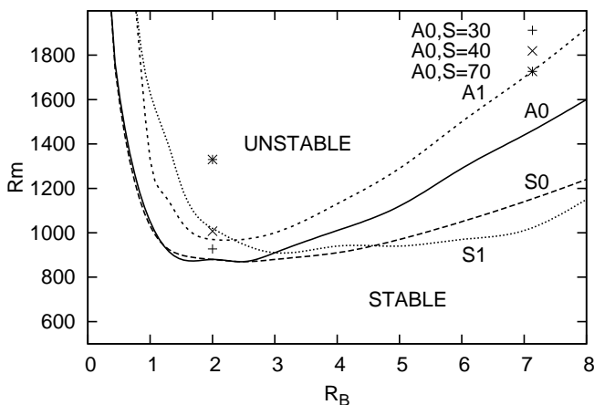
Fig. 1. Stability curves for the axisymmetric (S0 and A0) and non-axisymmetric (S1 and A1) modes. The single points belong to the system where the flow equation was treated in addition to the induction equation.
