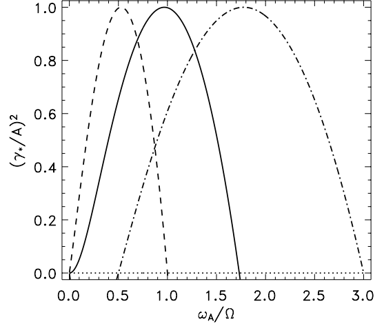
Fig. 1. The growth rates, \gamma_* = \gamma + \eta k^2 in units of A=q\Omega/2 as functions of the normalized field strength for MRI alone (full line) and MRI modified by the Hall effect of positive fields ( \beta = 1 , dashed line) and negative fields ( \beta = -1 , dashed-dotted). Pm = 1.
