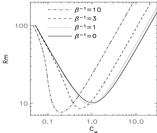
Fig. 5. The same as in Fig. 3 but for the full equation system. The Hall effect increases the minimum Rm. The solid curve for \beta \rightarrow \infty is identical to the lower curve in Fig. 3. For increasing Rm the lower limit for the magnetic field becomes smaller and smaller.
