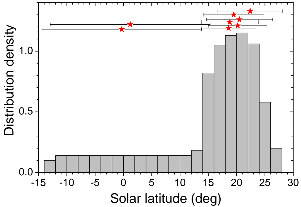
Fig. 3.— An example of the sunspot latitudinal distribution for Jul-Dec 1793, with 2^\circ latitudinal bins. Stars with error bars denote latitudes of individual spots as defined from Staudacher’s drawings. The histogram depicts the density of the latitudinal distribution of sunspots per 2^\circ bins per half-year computed by including the uncertainties.
