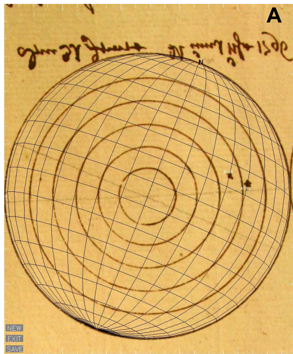
Fig. 2.— An example of drawings of sunspots on the solar disc made by Staudacher in Nürnberg, Germany at 1 p.m. local time on January 31, 1796. The image is mirrored to correspond to the real view to the solar disc. The heliographical grid has been included during the image processing (Arlt 2009a).
