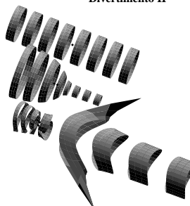
We show the stereoscopic aberration of a cylinder. First we draw eight segments at any given instant in the form in the middle. If the eyes are oriented across, the moving observer sees the lower form (in both cases, the velocity is 0.7c ). The contraction apparent in the form in the middle is the immediate expression of the Lorentz contraction of the distance of the eyes.
