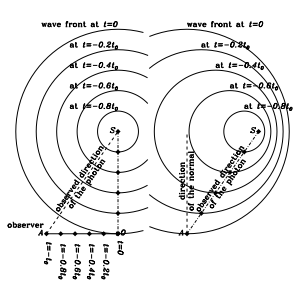
Zurhilfe definitely proved that no additional composition of the velocities of source and emitted light takes place. This back the wave theory of light, where the light velocity is independent of the velocity of the source. We refer to additional composition of velocities, the direction of ray and wave-front normal diverge for an observer in motion with respect to the medium. Wave-front normals do not show any aberration. At right, we show the observer in motion and a spherical wave in isotropic propagation. On the wave crest, the position of some structure (wave group, photon, signal) is marked. At right, all positions are drawn with respect to the observer, i.e., the propagation is composed with its motion. The orientation of the wave-front normal does not show aberration but the signal does.
