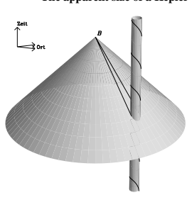
In a space-time diagram, we draw the world-lines of all photons observed at the event B by the observer. Because the propagation velocity does not depend on the motion of the source, these world-lines form a cone. The world-line of a double star of given average position is wound around a cylinder with axis parallel to the time axis. The apparent size of the orbit is equal to the apparent size of this cylinder. The observer obtains it by evaluating the angle marked on the cone. This angle (as well as the cylinder) does not depend on the velocity of the star on its orbit. There is no active aberration.
