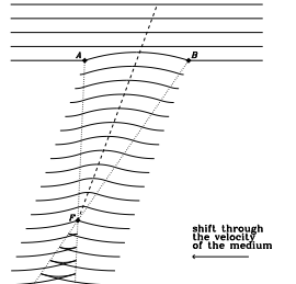
We see the motion of the wave front as constructed by Huygens's method. This motion is decelerated in the aperture lens and reaches a focus F' . The wave fronts are shifted to the left with progressing time. The focus is found in the position expected by the particle-type aberration argument.
