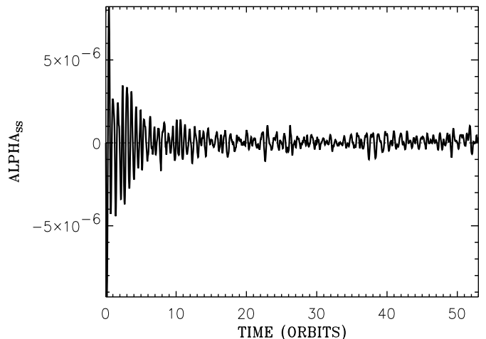
Fig. 2. Shakura-Sunyaev parameter \alpha_{SS} from the same model as in Fig. 1 (Model I). Times are again in orbital periods of the inner boundary of the domain
