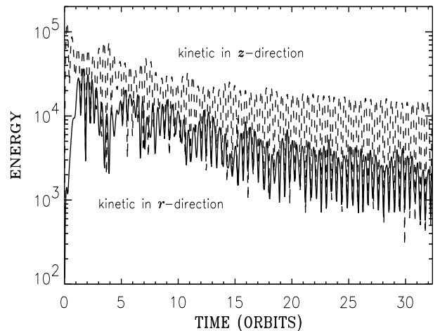
Fig. 4. Kinetic energies in the vertical (dashed) and radial (solid) components for the model with m = 200 in the initial perturbation (Model IV). The resolution of the computational domain is 31 \times 61 \times 701
