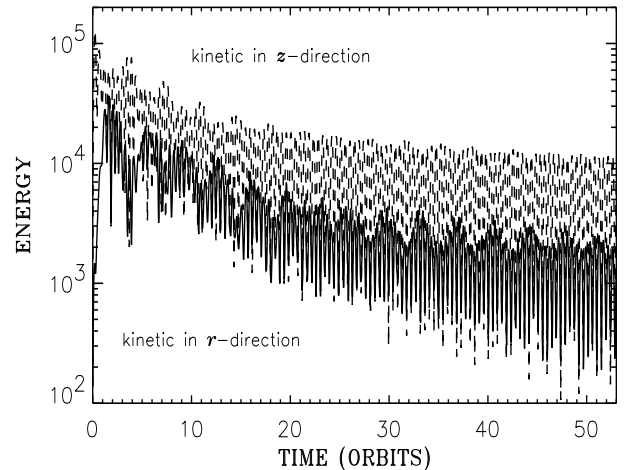
Fig. 1. Kinetic energies in the vertical and radial components of the flow from the run with 31 \times 61 \times 351 grid points (Model I). The solid line is the energy of the r -direction, the dashed line that of the z -direction. Times are given in revolutions of the inner boundary of the computational domain
