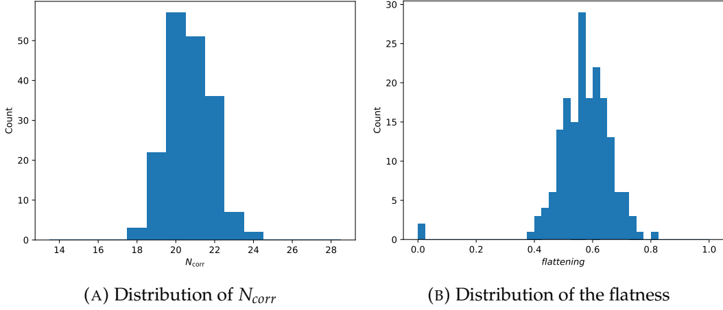
FIGURE 4.26: Histogram of the distribution of the minimum flatness and maximum N_{corr} of the 180 randomly created systems rotated 100 times
