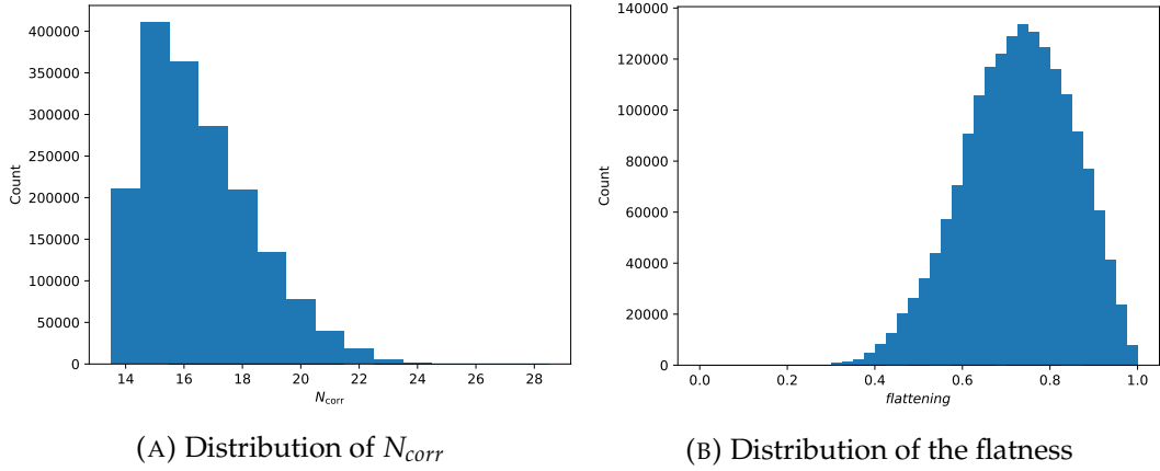
FIGURE 4.10: Histogram of the distribution of the calculated values of the 180 simulated systems rotated 10000 times
