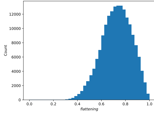
(B) Distribution of the flatness
