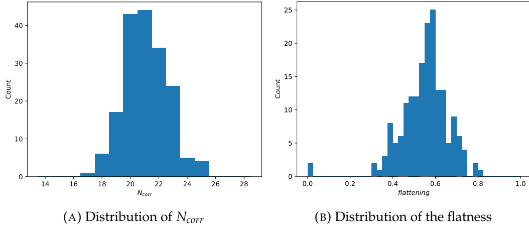
FIGURE 4.28: Histogram of the distribution of the minimum flatness and maximum N_{corr} of the 180 simulated systems rotated 100 times
