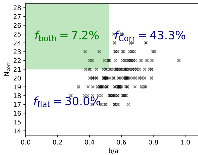
FIGURE 4.34: calculated optimal pairs for the 180 simulated systems with 1000 rotations.
