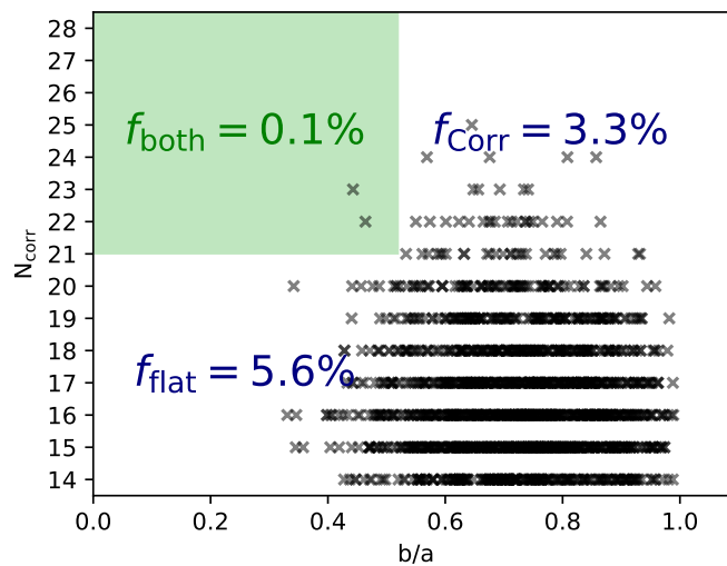
FIGURE 4.2: Every result calculated for the 180 simulations with 10 rotations. both results were from the same POV
