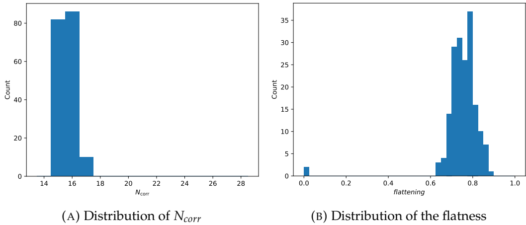
FIGURE 4.11: Histogram of the distribution of the calculated average of the 180 randomly created systems rotated 100 times
