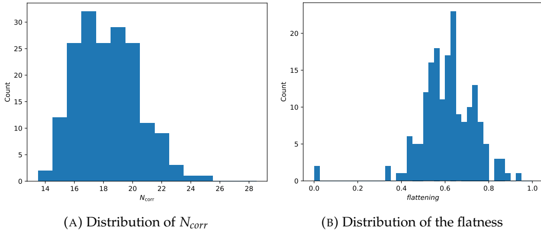
FIGURE 3.6: Example plot of the distribution of minimum flatness and maximum N_{corr}
