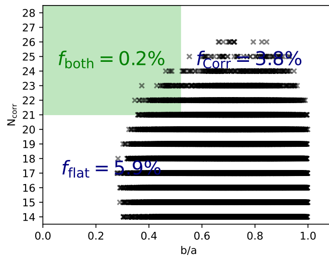
FIGURE 4.4: Every result calculated for the 180 simulations with 1000 rotations. both results were from the same POV
