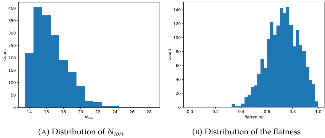
FIGURE 4.7: Histogram of the distribution of the calculated values of the 180 simulated systems rotated 10 times
