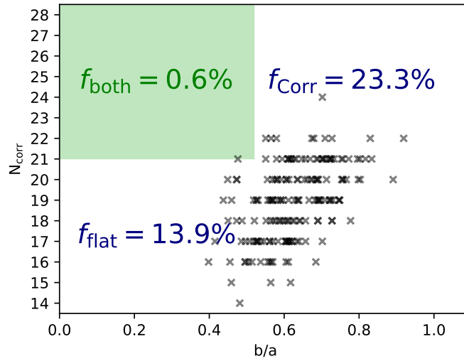
FIGURE 4.31: calculated optimal pairs for the 180 randomly created systems with 100 rotations.
