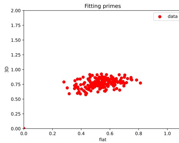
FIGURE 4.45: calculated 3D flatness over 2D flatness for the 180 simulated systems with 10000 rotations
