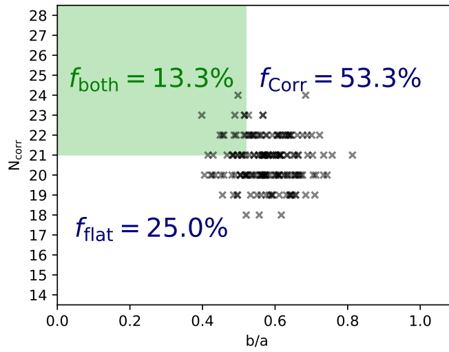
FIGURE 4.21: calculated extremes for the 180 randomly created systems with 100 rotations. the results are not from the same POV
