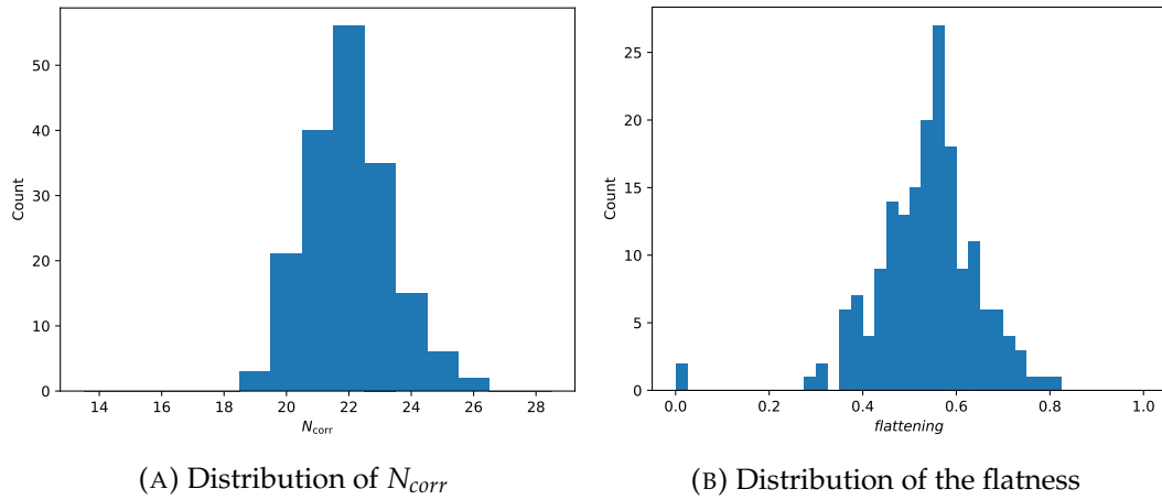
FIGURE 4.29: Histogram of the distribution of the minimum flatness and maximum N_{corr} of the 180 simulated systems rotated 1000 times
