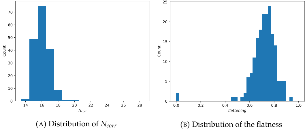
FIGURE 3.7: Example plot of the distribution of the average values of flatness and maximum N_{corr} for each simulated system
