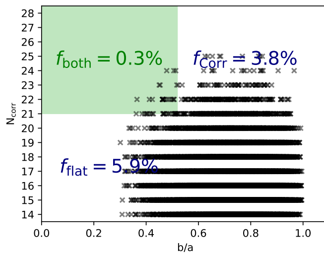
FIGURE 4.3: Every result calculated for the 180 simulations with 100 rotations. both results were from the same POV
