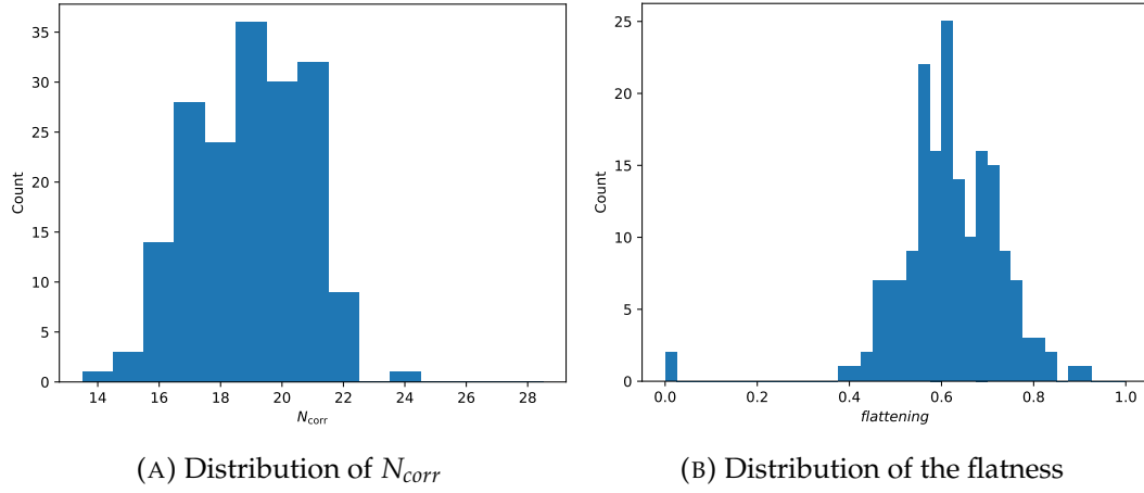
FIGURE 4.36: Histogram of the distribution of the optimal flatness and maximum N_{corr} of the 180 randomly created systems rotated 100 times
