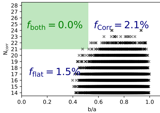
FIGURE 4.1: Every result calculated for the 180 randomly created systems with 100 rotations. both results were from the same POV
