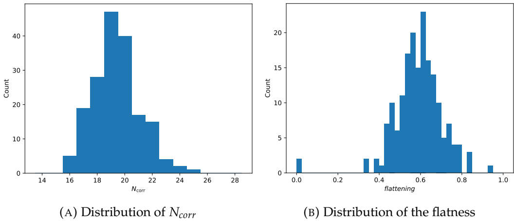
FIGURE 3.4: Example plot of the distribution of minimum flatness and maximum N_{corr}
