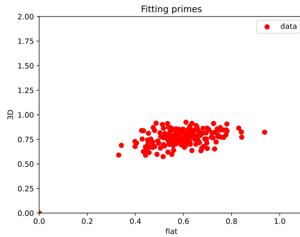
FIGURE 4.42: calculated 3D flatness over 2D flatness for the 180 simulated systems with 10 rotations
