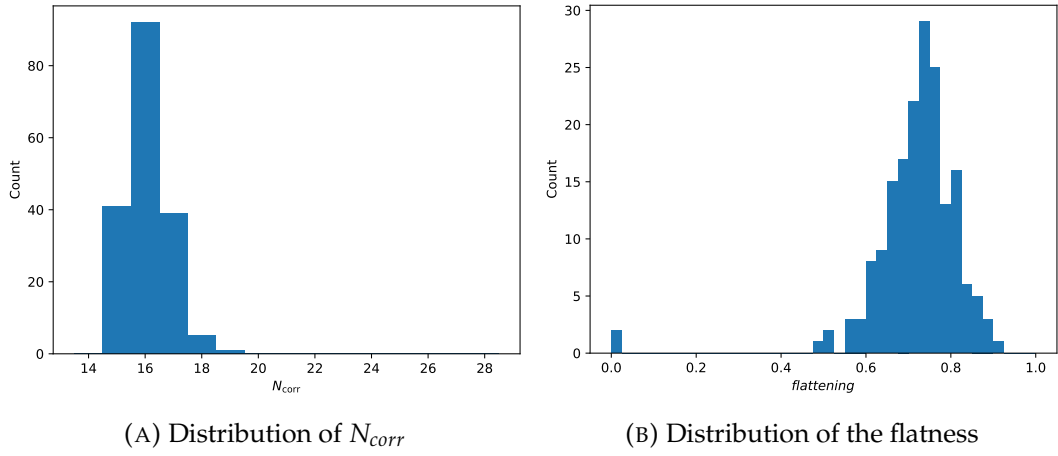
FIGURE 4.14: Histogram of the distribution of the calculated average of the 180 simulated created systems rotated 1000 times
