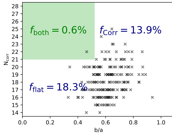
FIGURE 4.32: calculated optimal pairs for the 180 simulated systems with 10 rotations.
