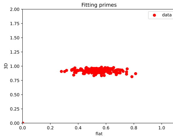
FIGURE 4.41: calculated 3D flatness over 2D flatness for the 180 randomly created systems with 100 rotations
