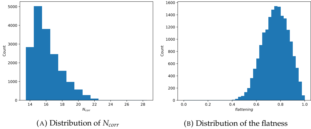
FIGURE 4.6: Histogram of the distribution of the calculated values of the 180 randomly created systems rotated 100 times
