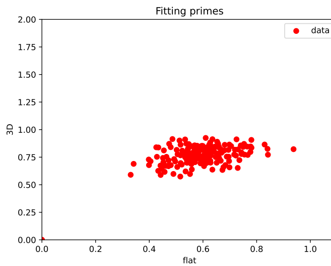
FIGURE 3.9: Example plot of 2D flatness on the x-axis and the 3D flatness on the y-axis
