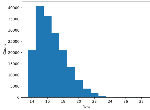
(A) Distribution of N_{corr}
