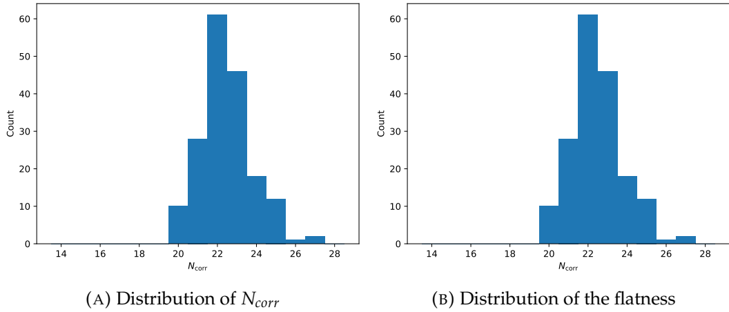
FIGURE 4.30: Histogram of the distribution of the minimum flatness and maximum N_{corr} of the 180 simulated systems rotated 10000 times
