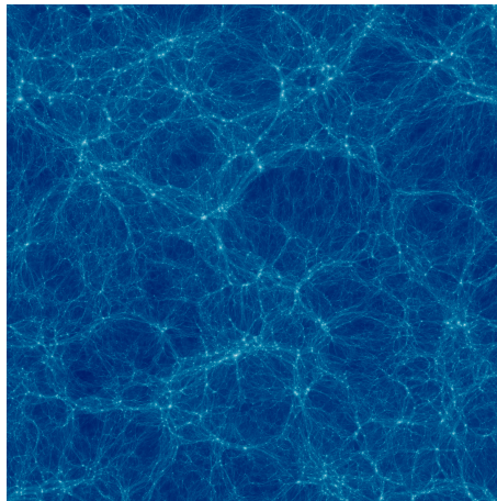
FIGURE 2.3: an Illustration of a simulated cosmic web [5]
