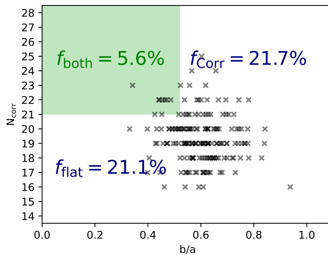
FIGURE 4.22: calculated extremes for the 180 simulated systems with 10 rotations. the results are not from the same POV
