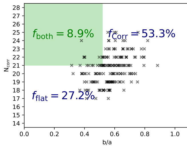
FIGURE 4.35: calculated optimal pairs for the 180 simulated systems with 10000 rotations.
