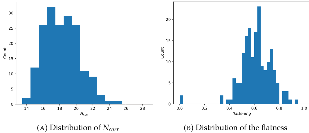
FIGURE 4.37: Histogram of the distribution of the optimal flatness and maximum N_{corr} of the 180 simulated systems rotated 10 times
