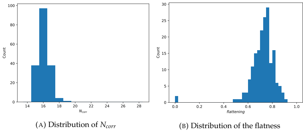
FIGURE 4.15: Histogram of the distribution of the calculated average of the 180 simulated created systems rotated 10000 times
