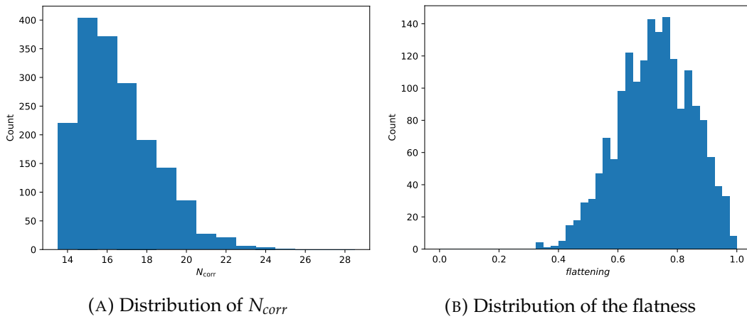
FIGURE 3.2: Example plot of all calculated values. x-axis shows the calculated flatness or N_{corr} , while the y-axis shows from how many points of view we get the same value
