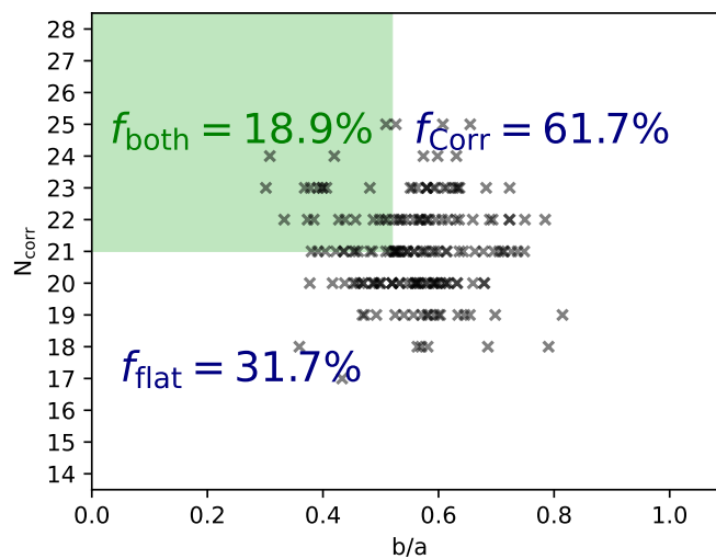
FIGURE 4.23: calculated extremes for the 180 simulated systems with 100 rotations. the results are not from the same POV
