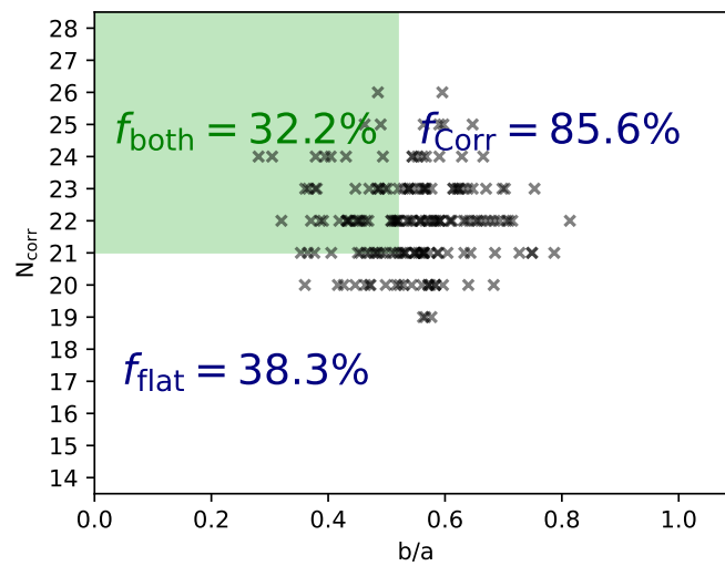
FIGURE 4.24: calculated extremes for the 180 simulated systems with 1000 rotations. the results are not from the same POV
