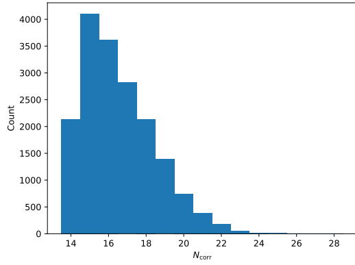
(A) Distribution of N_{corr}
