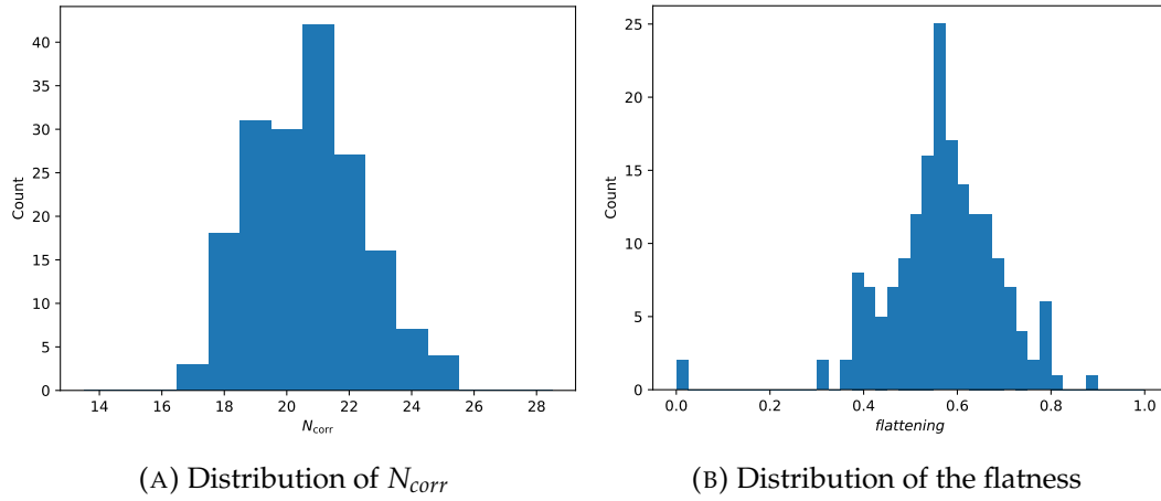
FIGURE 4.40: Histogram of the distribution of the optimal flatness and maximum N_{corr} of the 180 simulated systems rotated 10000 times
