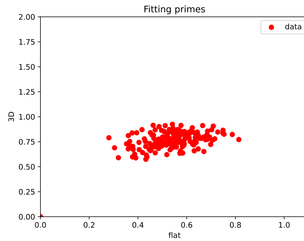
FIGURE 4.44: calculated 3D flatness over 2D flatness for the 180 simulated systems with 1000 rotations
