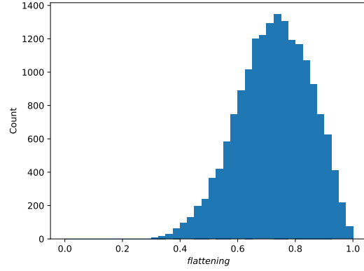
(B) Distribution of the flatness
