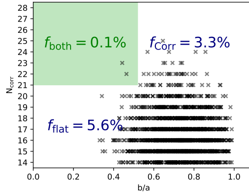
FIGURE 3.1: Example plot of all calculated values for flatness on the x-axis and N_{corr} on the y-axis. We used 180 simulations and a certain number of rotations to change the POV
