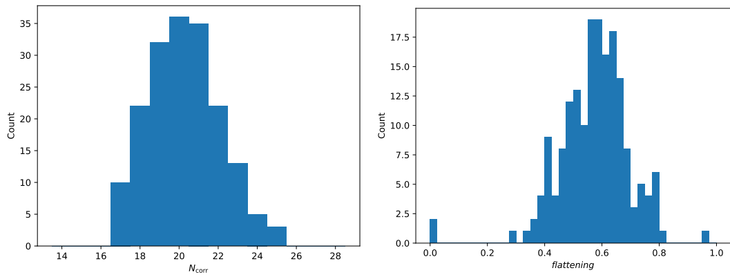
(B) Distribution of the flatness
