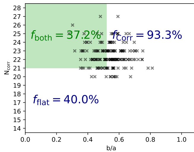
FIGURE 4.25: calculated extremes for the 180 simulated systems with 10000 rotations. the results are not from the same POV
