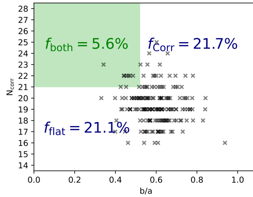
FIGURE 3.3: Example plot of all the minimum and maximum for every simulation. It is important to note, that the flatness and N_{corr} are from the same system but not the same point of view. Therefore, there are 180 results illustrated in this plot.
