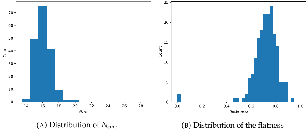
FIGURE 4.12: Histogram of the distribution of the calculated average of the 180 simulated created systems rotated 10 times
