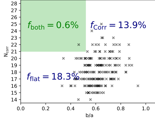
FIGURE 3.5: Example plot of the highest possible N_{corr} and lowest possible flatness from the same POV for each simulation.
