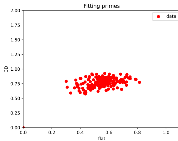
FIGURE 4.43: calculated 3D flatness over 2D flatness for the 180 simulated systems with 100 rotations
