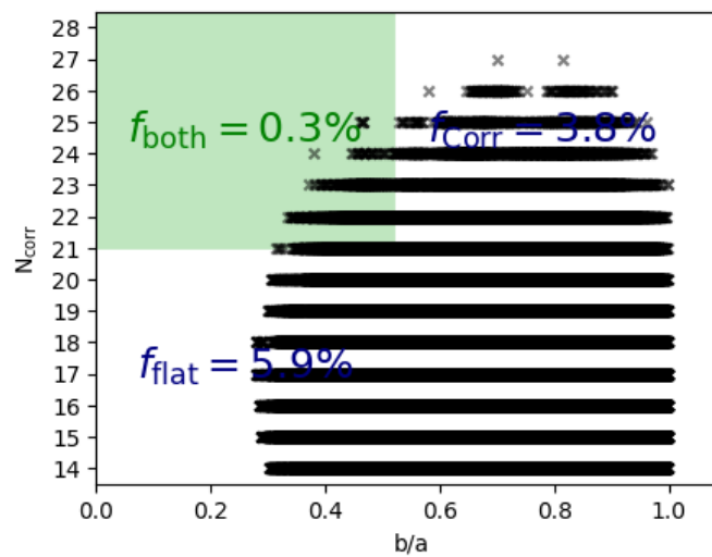
FIGURE 4.5: Every result calculated for the 180 simulations with 10000 rotations. both results were from the same POV
