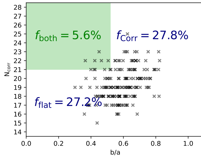
FIGURE 4.33: calculated optimal pairs for the 180 simulated systems with 100 rotations.
