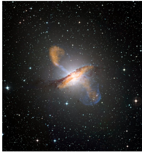
FIGURE 2.2: An illustration of Centaurus A[3]
