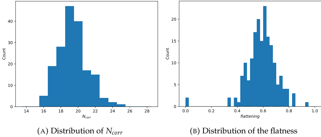
FIGURE 4.27: Histogram of the distribution of the minimum flatness and maximum N_{corr} of the 180 simulated systems rotated 10 times
