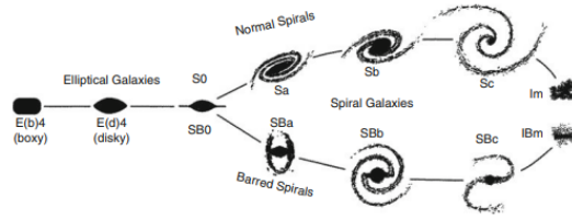
FIGURE 2.1: 'Hubble's 'tuning fork' for galaxy classification. Adapted from: J. Kormendy & R. Bender 1996, A Proposed Revision of the Hubble Sequence for Elliptical Galaxies, ApJ 464, L119, Fig. 1.c AAS. Reproduced with permission'[2]
