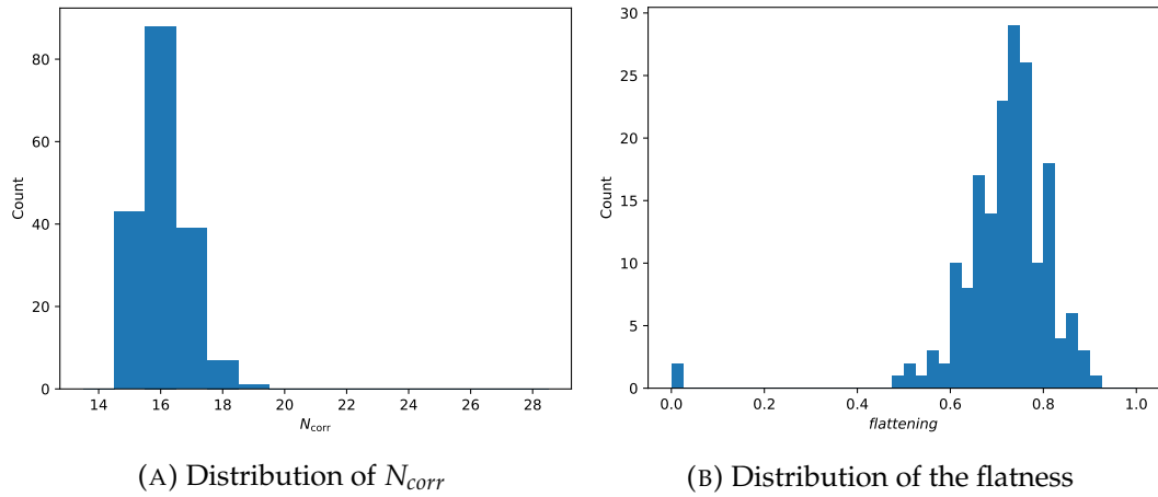
FIGURE 4.13: Histogram of the distribution of the calculated average of the 180 simulated created systems rotated 100 times
